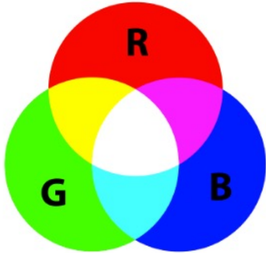
Figure 2: The mechanism of additive color synthesis. LIGO Hanford is assigned to red, LIGO Livingston to green and Virgo to blue. A triple coincidence will appear in white, while a double coincidence in yellow, magenta or cyan, depending on which couple of detectors is involved.
