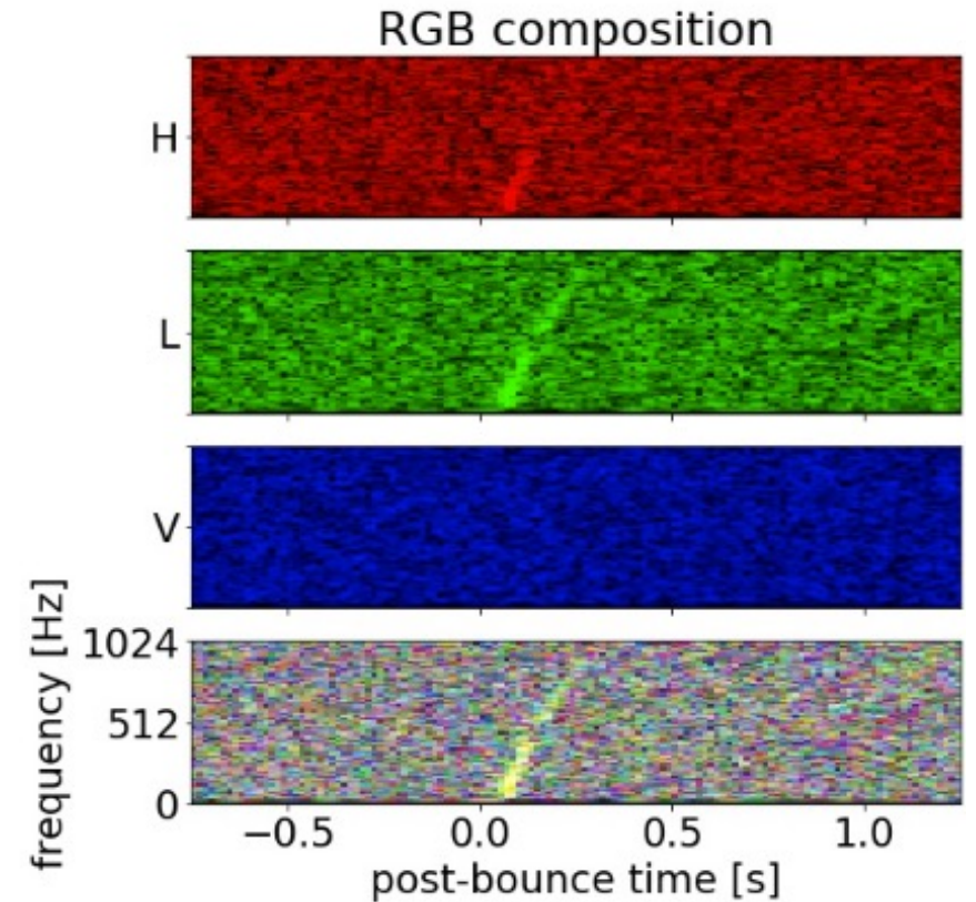
Figure 3: From the top; the spectrogram of LIGO Hanford is red, then that of LIGO Livingston is green and Virgo is blue. At the bottom: the RGB image obtained by stacking the previous three spectrograms. In this case, the signal is present just in Hanford and Livingston so that the combined signal at the bottom is in yellow.
