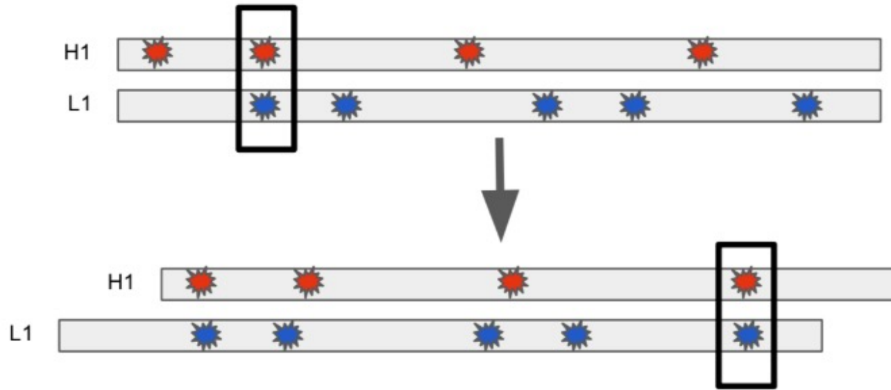
Timeslides for measuring the GW background.
